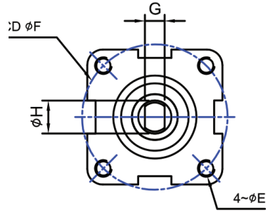
Mounting Dimensions
