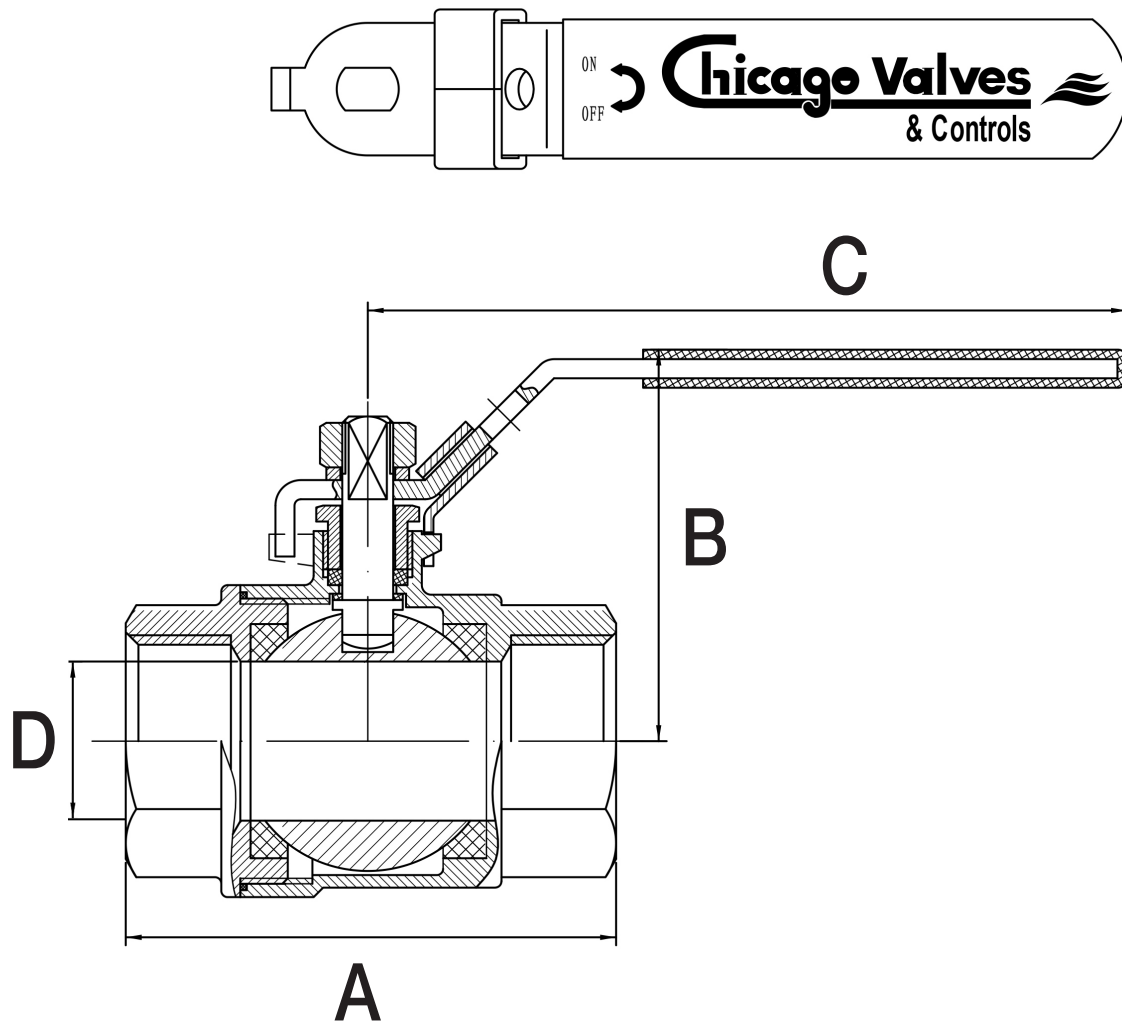
DIMENSIONS (INCHES)
